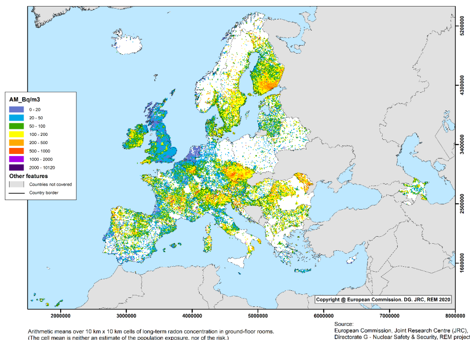
European Indoor Radon Map, December 2020
