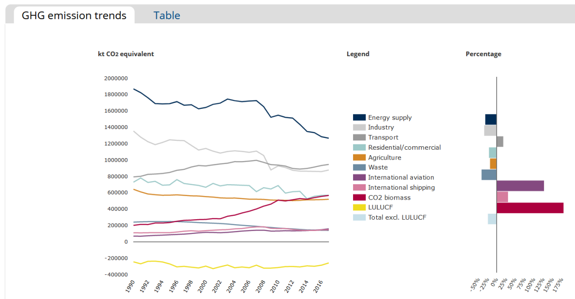
Fig. 2: Greenhouse gas emissions by aggregated sector
